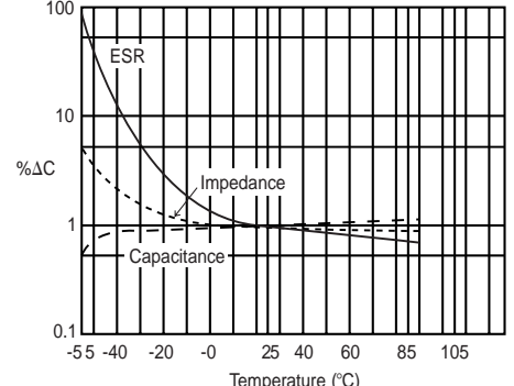
Temperature Characteristics - 4600 \mu\text{F} 100 Vdc
